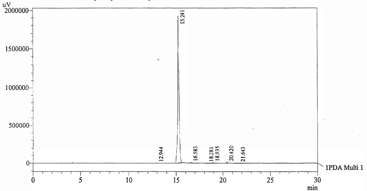
Chromatogram 2-Hydroxychalcone D:\promonence\Data\2013JUNE-2013\040613K.lcd
